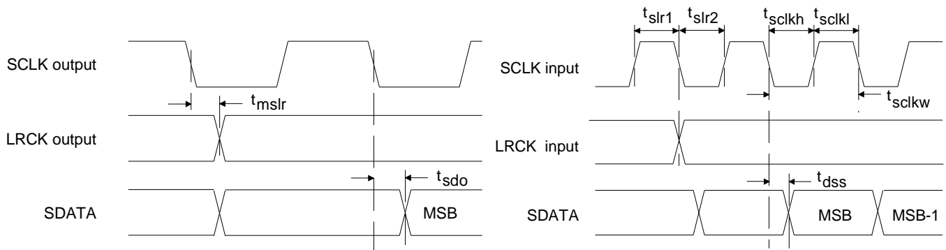
SCLK to SDATA & LRCK - MASTER mode Serial Data Format, DFS high I 2 S compatible
