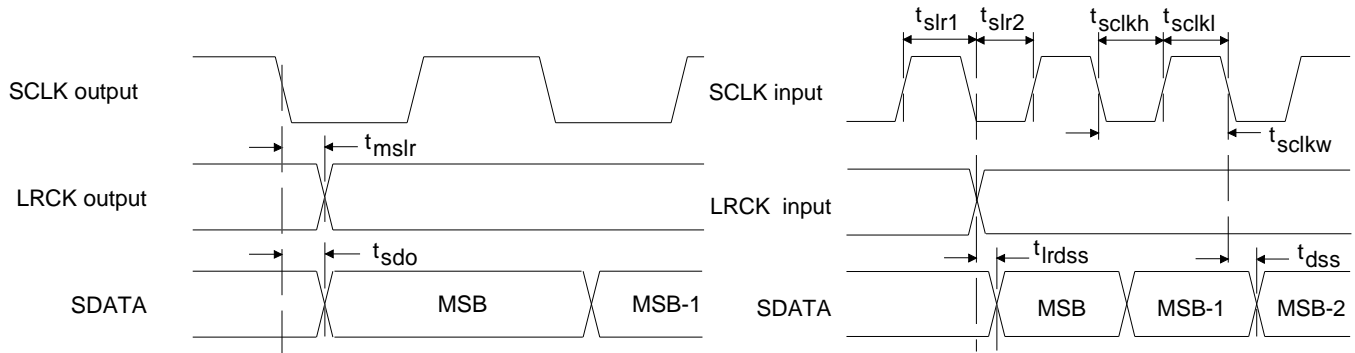
SCLK to SDATA & LRCK - MASTER mode Serial Data Format, DFS low
