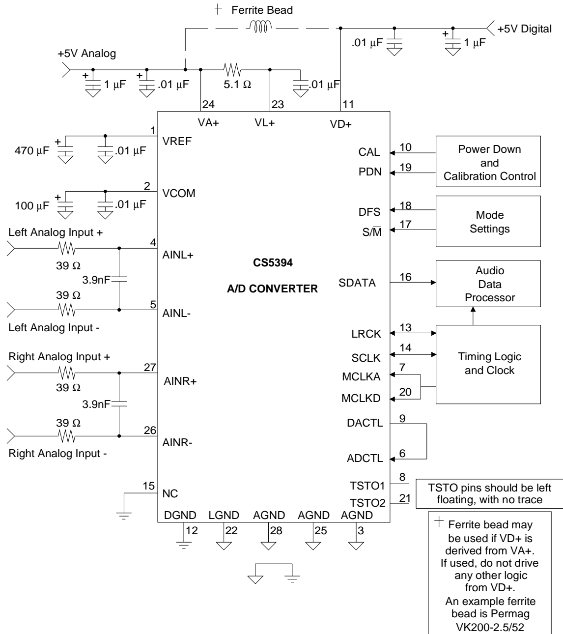
Figure 1. Typical Connection Diagram
